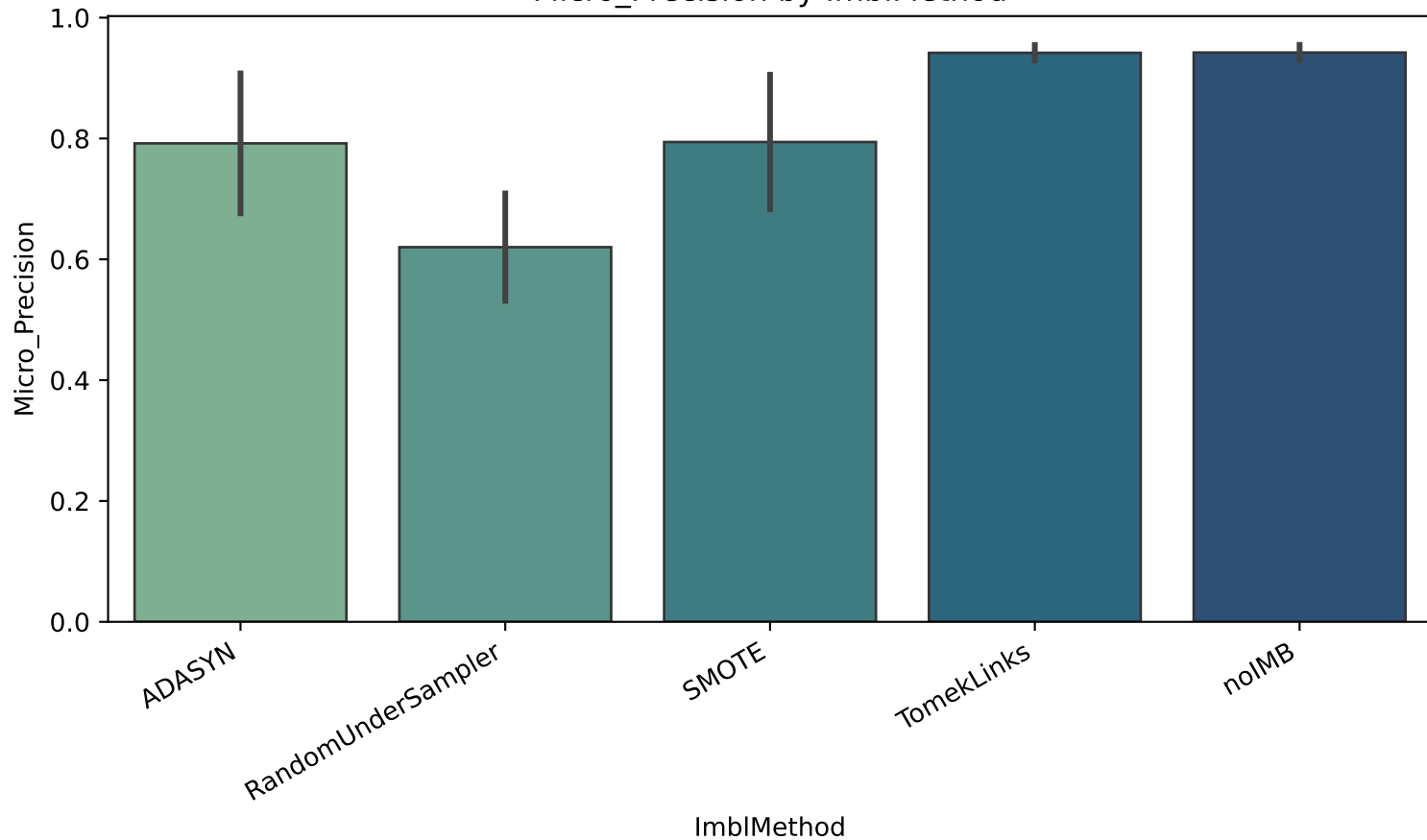
Micro_Precision by ImblMethod
